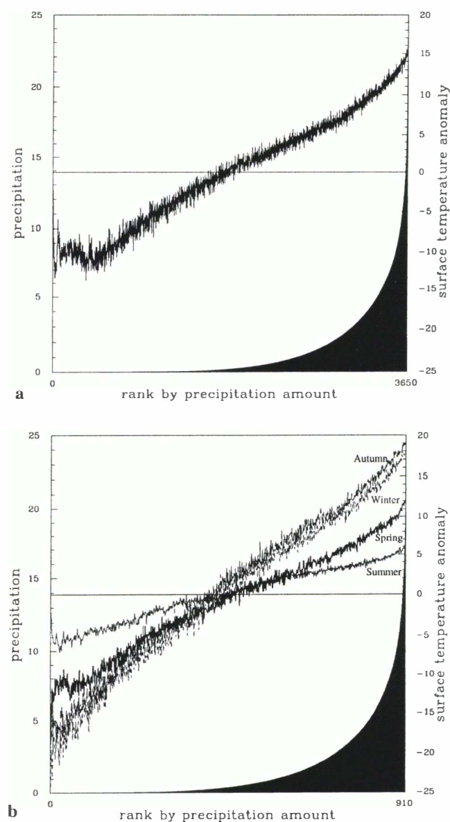
Fig. 3. Mean precipitation amount (shaded region) and corresponding mean surface-temp. The x axis is ranked by precipitation amount from lowest to highest for (a) all data (3650 days) and (b) seasonal comparison (910 days). Surface-temperature anomaly is marked on the right axis in °C, and precipitation is on the left axis in \text{mm d}^{-1} .
