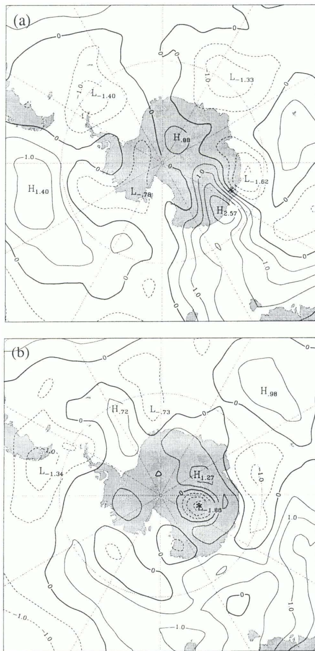
Fig. 1. MSLP anomaly on days with > 5 \text{ mm} precipitation for (a) Casey and (b) Vostok locations. The contour interval is 0.5 \text{ hPa} and the zero contour is shown in bold.
